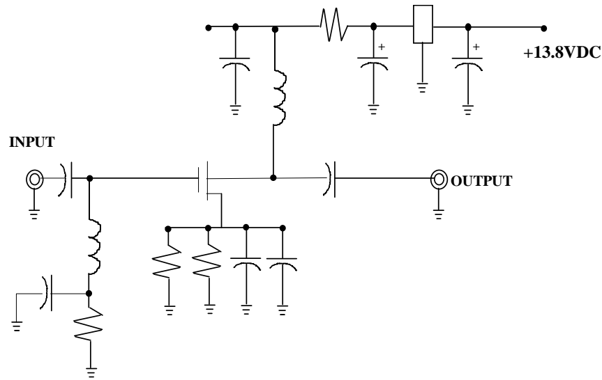
Schematic shown is the 15 dB gain, +30 IP3 output model.
