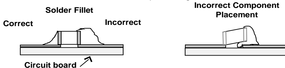
Figure 3. Proper SMD Assembly.
