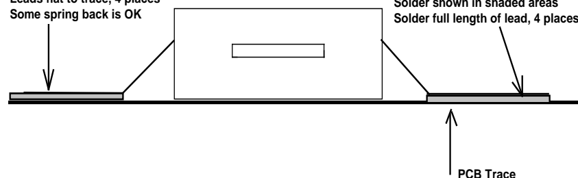
Typical side view of four leaded surface mounted device, lead bending close to body.
