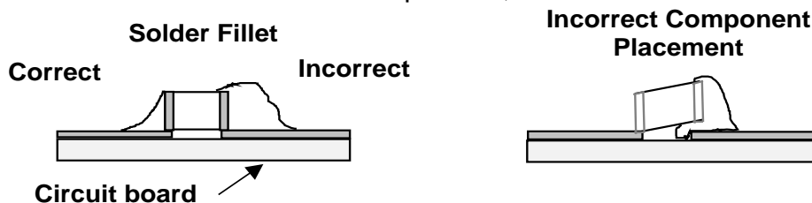
Figure 4. Proper SMD Assembly.
