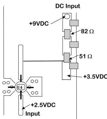
Figure 9. Resistor Network with Voltage Points
