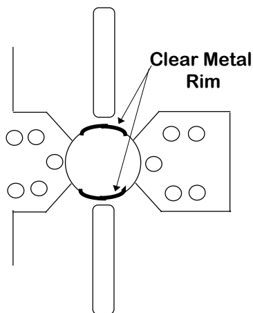
Figure 1. MMIC PC Board hole with metal rim
