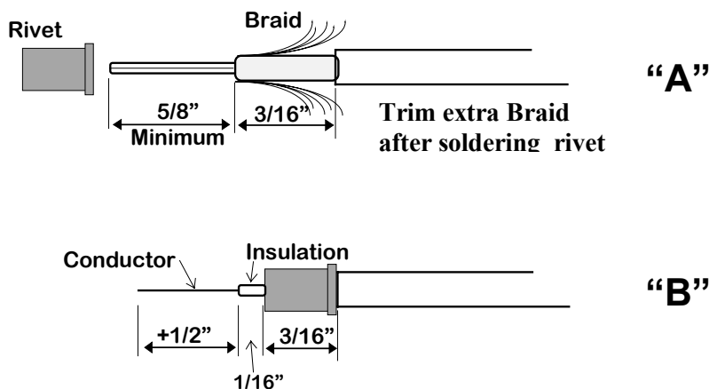
Figure 5. Prepped Coax details.
