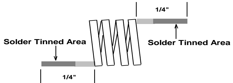
Top view of normally formed coil, (4 turns shown)
