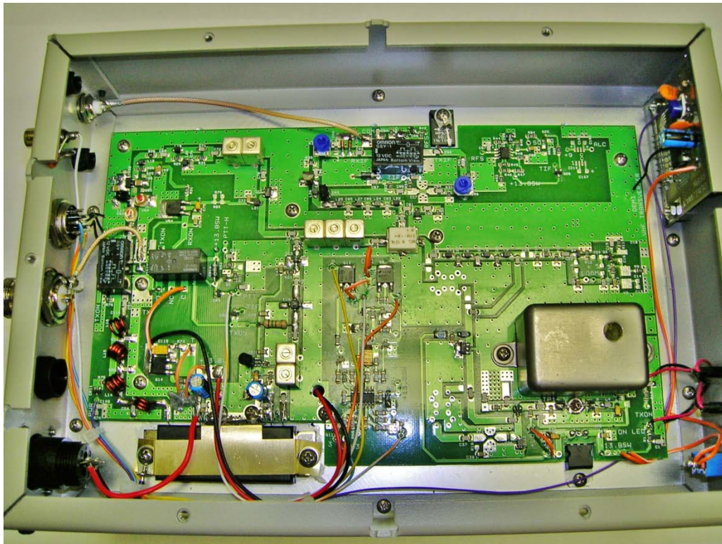
32. The inside view of completed transverter.
