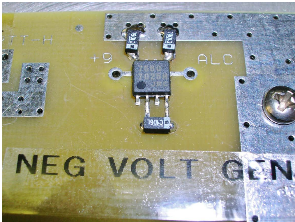
18. Negative Voltage generator installation on proto board.
