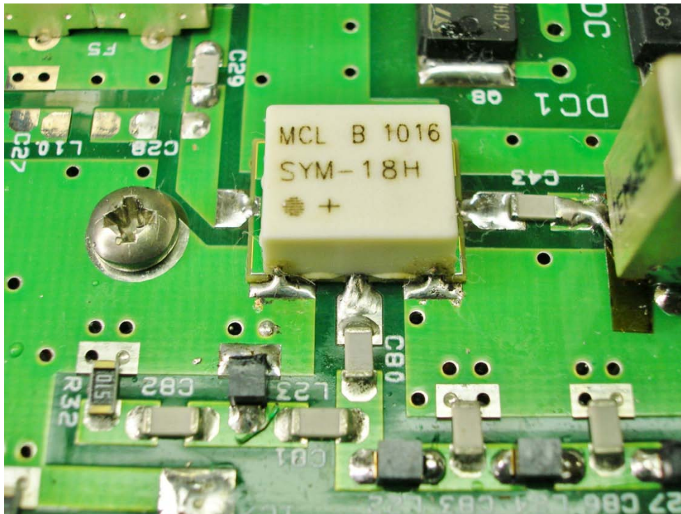
16. IF diplexer and PIN diode installation.
