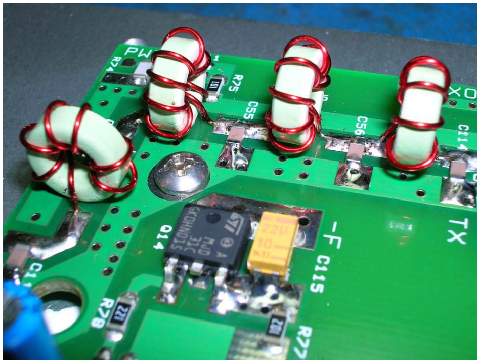
21. TX low pass filter, fan speed and power detect circuit.
