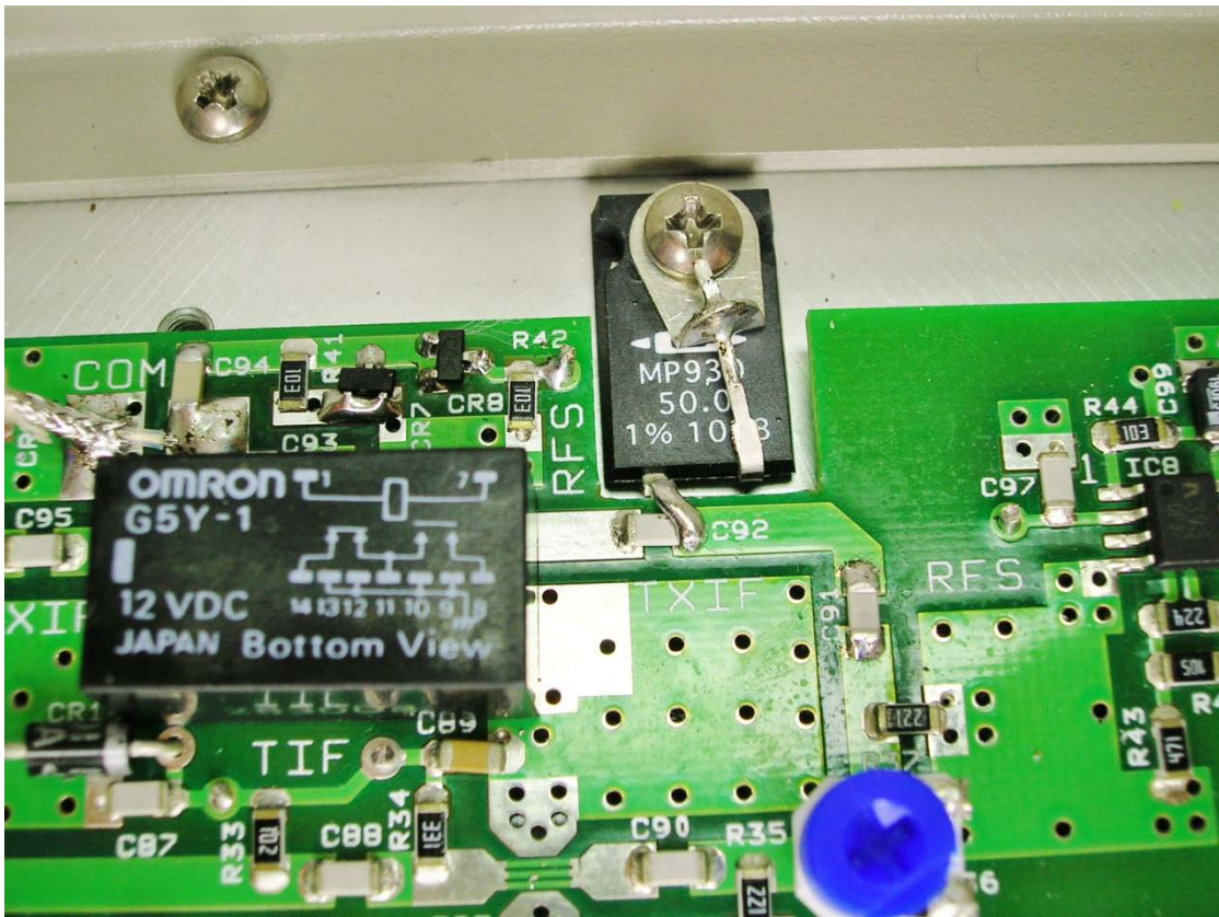
18. Negative Voltage generator installation on proto board.
