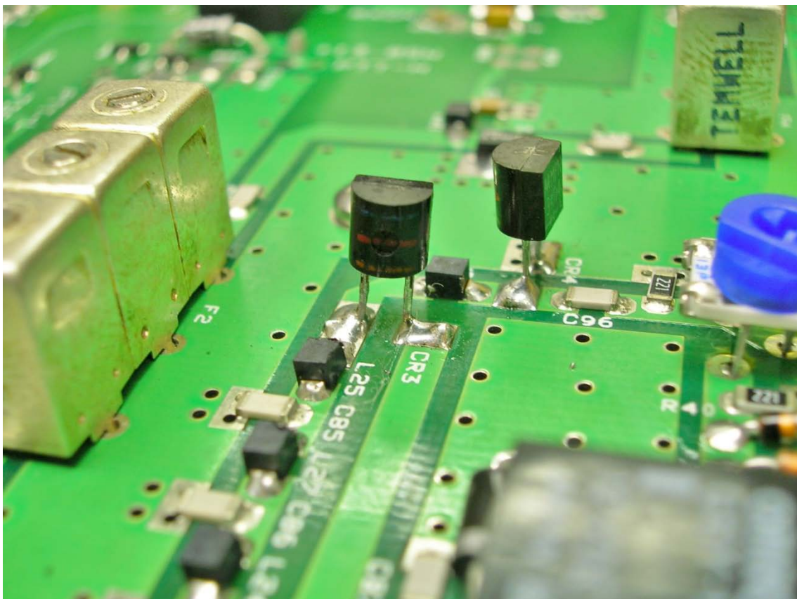
16. IF diplexer and PIN diode installation.
